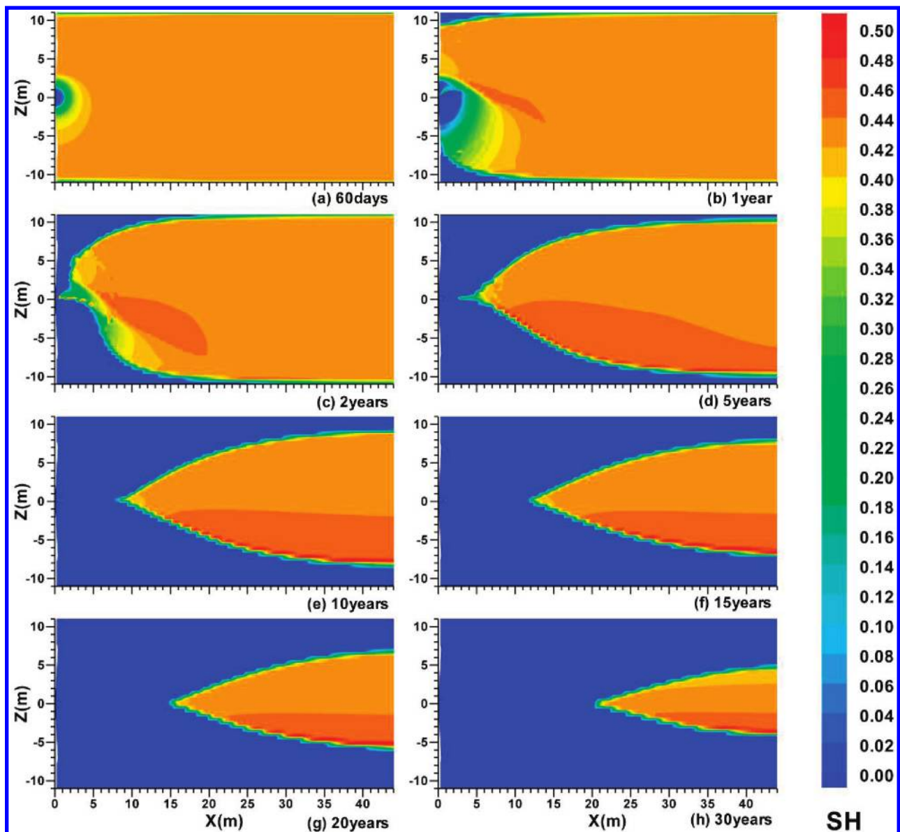
Figure 7. Evolution of spatial distribution of S_H when \Delta P_W = 0.2P_0 during gas production from the methane hydrate deposit at the SH7 Site of the Shenhu Area, South China Sea.
