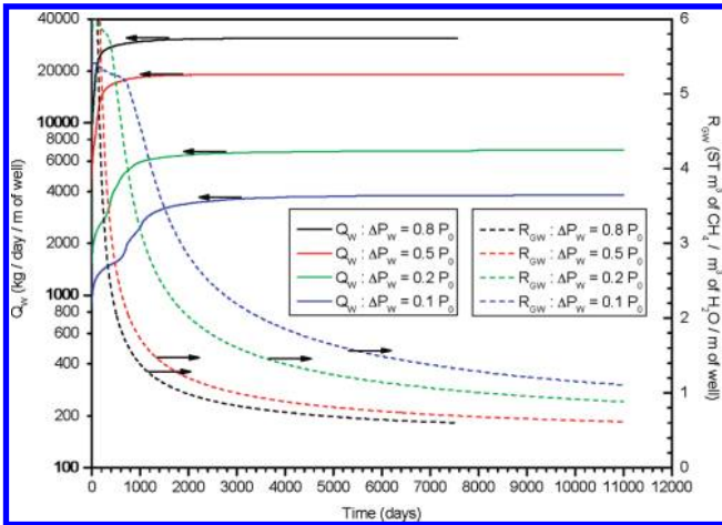
Figure 6. Evolution Q_W and R_{GW} using the depressurization method with \Delta P_W = 0.8P_0, 0.5P_0, 0.2P_0, and 0.1P_0, T_0 = 13.7 °C during gas production from the methane hydrate deposit in this study.
