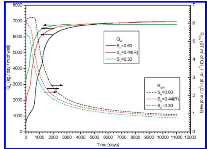
Figure 13. Sensitivity analysis: effect of S_{H0} on the evolution Q_W and R_{GW} when \Delta P_W = 0.2P_0 during gas production from the methane hydrate deposit at the SH7 Site of the Shenhu Area, South China Sea ( S_{H0} = 0.44 in the reference case).
