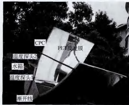
图 6 新型闷晒式太阳能热水器 Fig. 6 Novel integrated solar water heater with proposed collecting system
