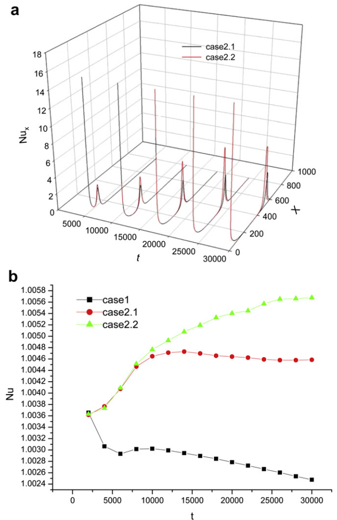
Fig. 6. (a) Comparison of local Nusselt number from cases of different bubble growth rate. (b) Effect of seed bubble growth on convective heat transfer (average Nusselt number).
